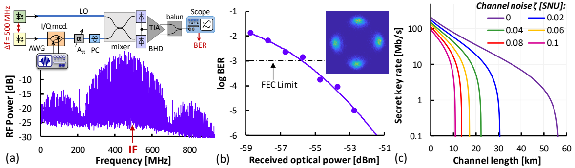
Fig. 3: (a) Heterodyned QPSK after coherent detection. (b) BER performance for 500 Mb/s QPSK reception. (c) Simulated secure-key rate for CV-QKD with untrusted receiver, based on the noise characteristics of the demonstrated CV receiver.
